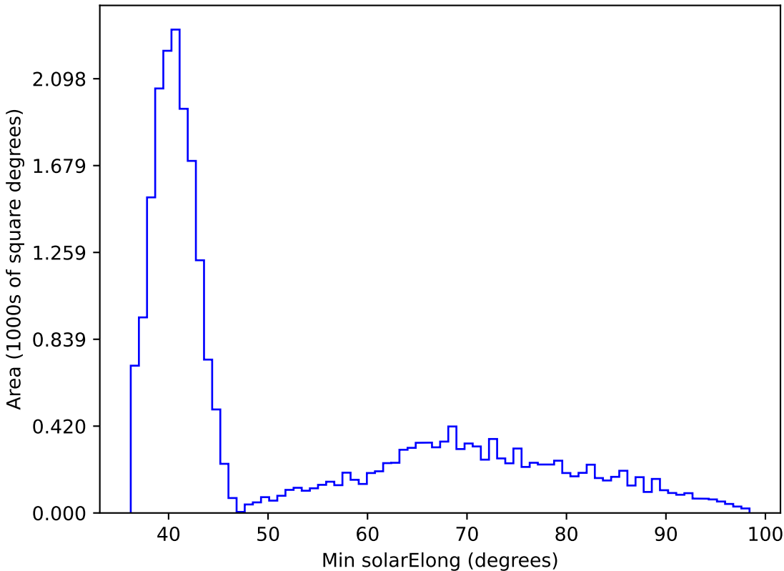
too_elab_r128_d3_gz_v3.4_10yrs All sky i band: Min solarElong
