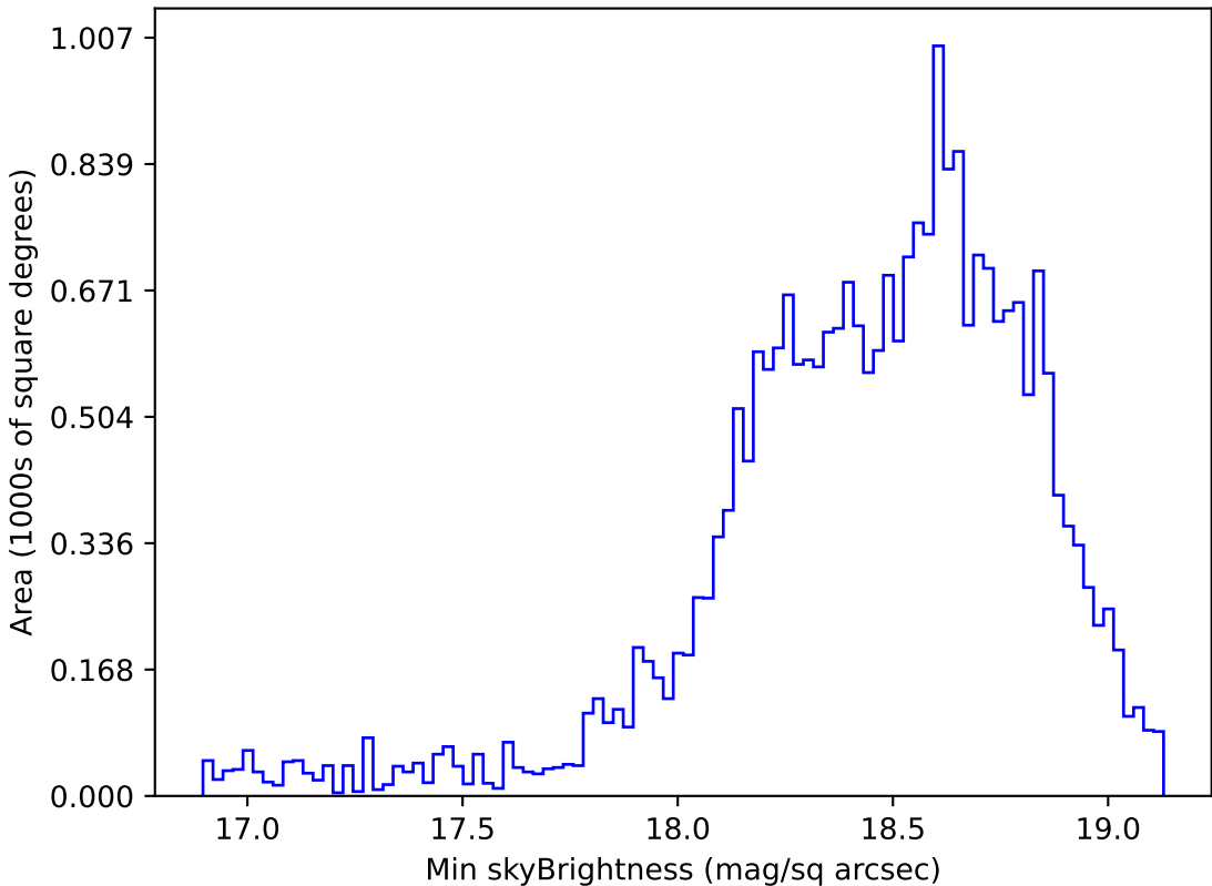
too_elab_r128_d3_gz_v3.4_10yrs Yr 1 z band: Min skyBrightness
