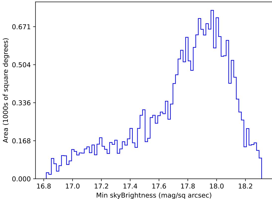
too_elab_r128_d3_gz_v3.4_10yrs Yr 1 y band: Min skyBrightness
