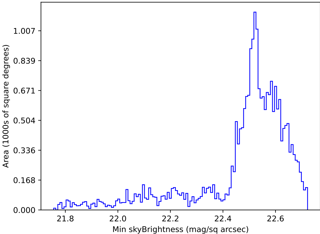
too_elab_r128_d3_gz_v3.4_10yrs Yr 1 u band: Min skyBrightness
