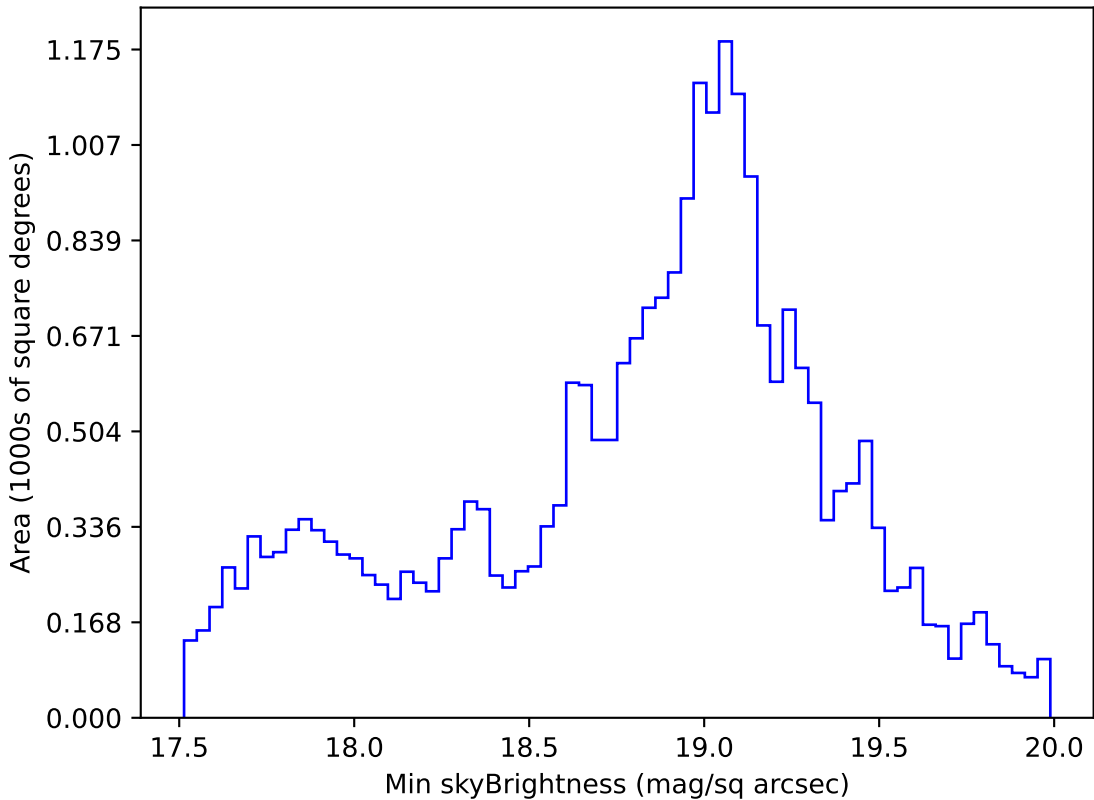
too_elab_r128_d3_gz_v3.4_10yrs Yr 1 i band: Min skyBrightness
