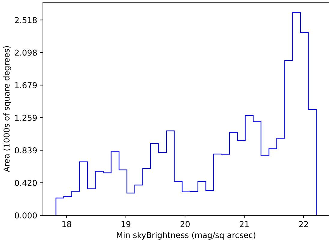
too_elab_r128_d3_gz_v3.4_10yrs Yr 1 g band: Min skyBrightness
