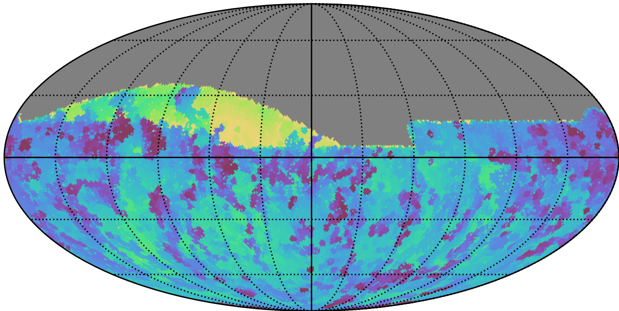
too_elab_r128_d3_gz_v3.4_10yrs Yr 1 all bands: Min skyBrightness
