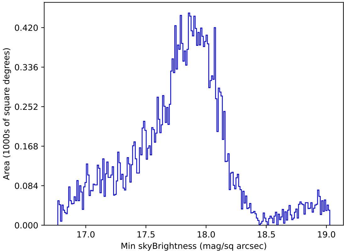
too_elab_r128_d3_gz_v3.4_10yrs Yr 1 all bands: Min skyBrightness
