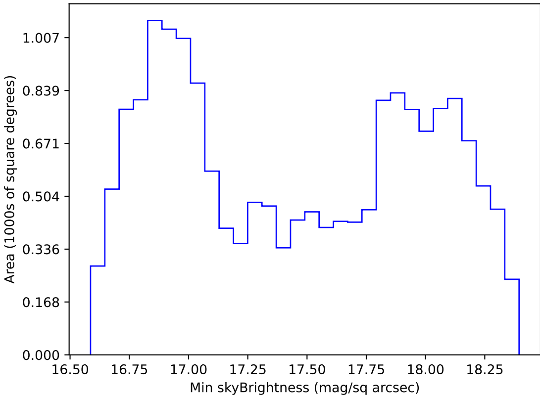
too_elab_r128_d3_gz_v3.4_10yrs WFD z band: Min skyBrightness
