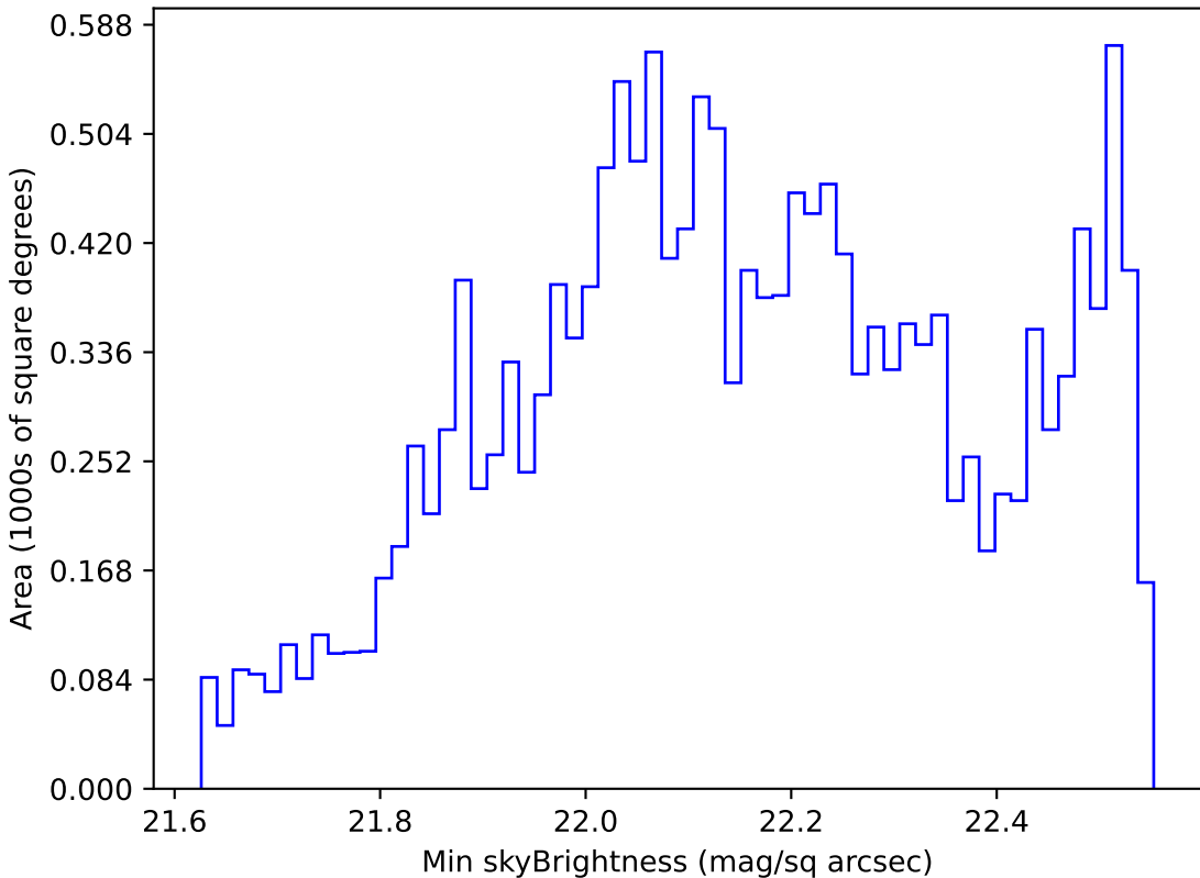
too_elab_r128_d3_gz_v3.4_10yrs WFD u band: Min skyBrightness
