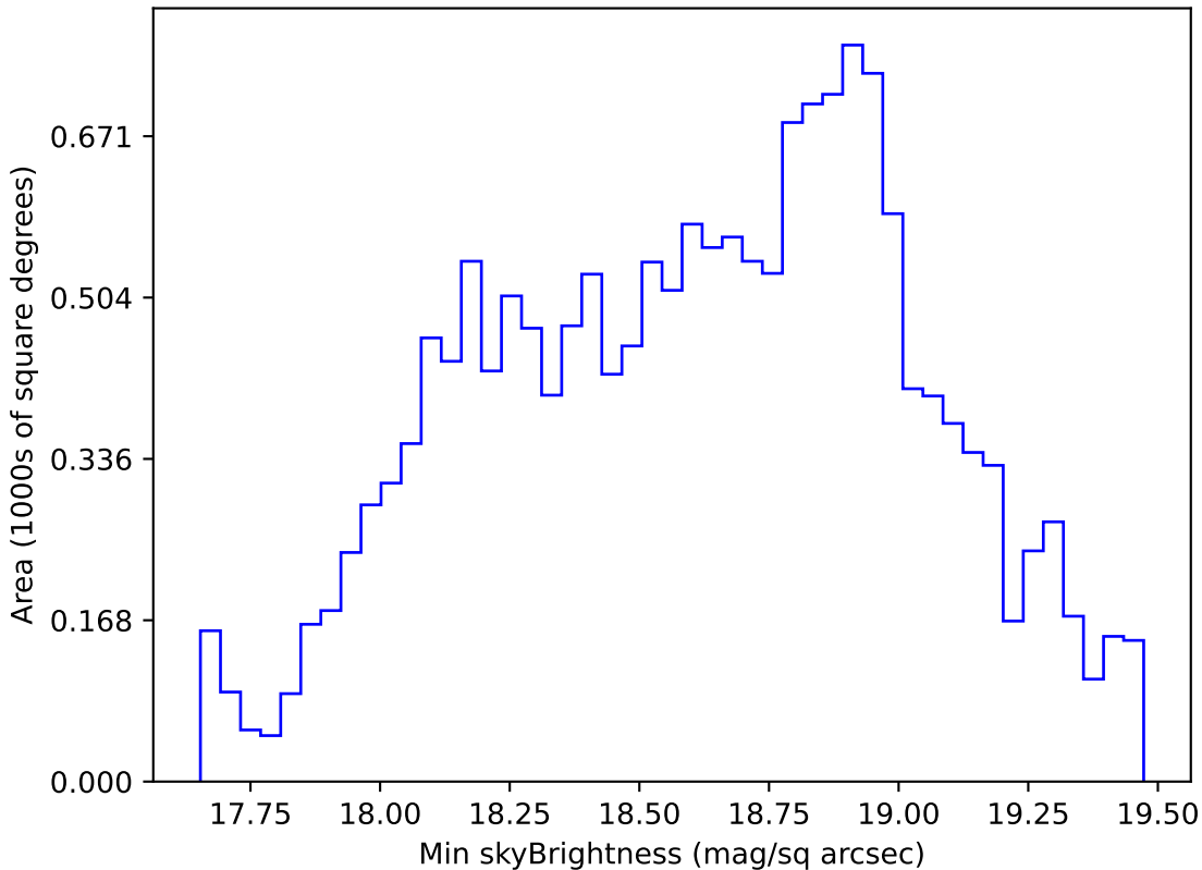
too_elab_r128_d3_gz_v3.4_10yrs WFD r band: Min skyBrightness
