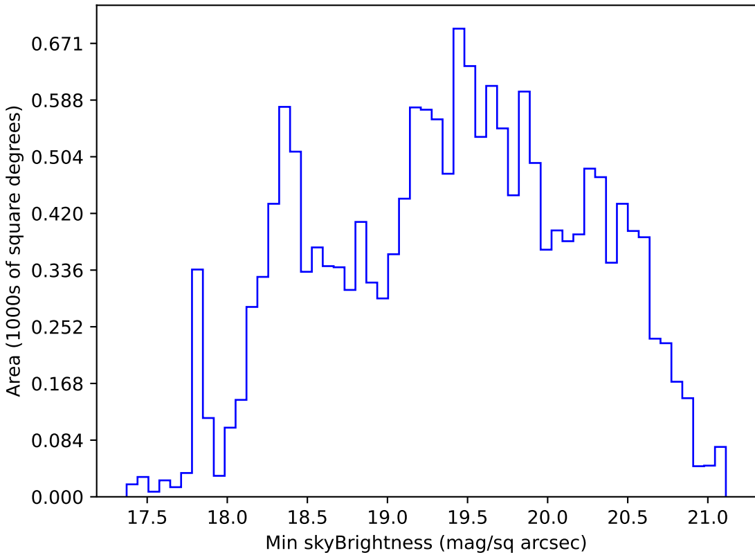
too_elab_r128_d3_gz_v3.4_10yrs WFD g band: Min skyBrightness
