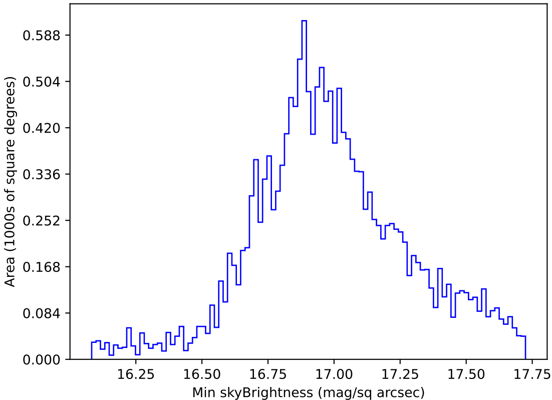
too_elab_r128_d3_gz_v3.4_10yrs WFD all bands: Min skyBrightness
