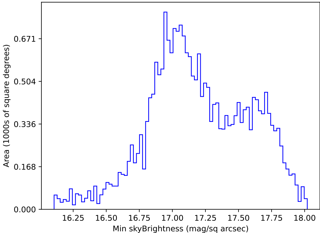
too_elab_r128_d3_gz_v3.4_10yrs All sky y band: Min skyBrightness
