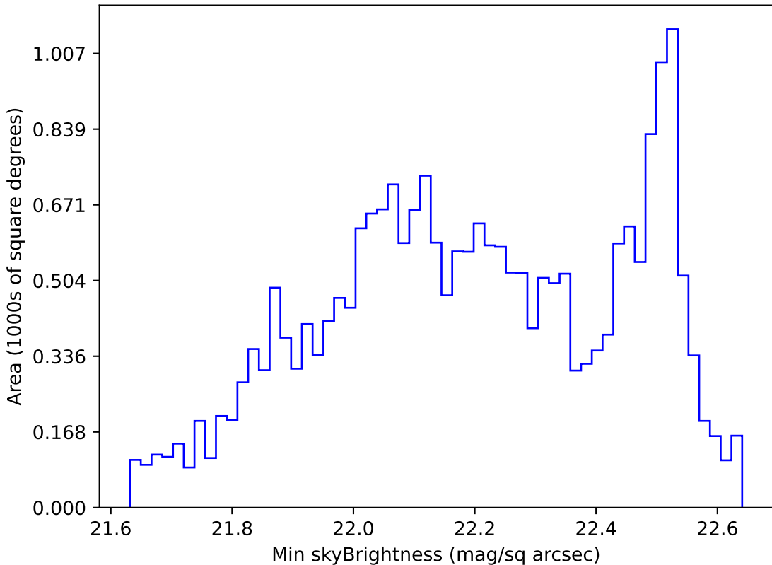
too_elab_r128_d3_gz_v3.4_10yrs All sky u band: Min skyBrightness
