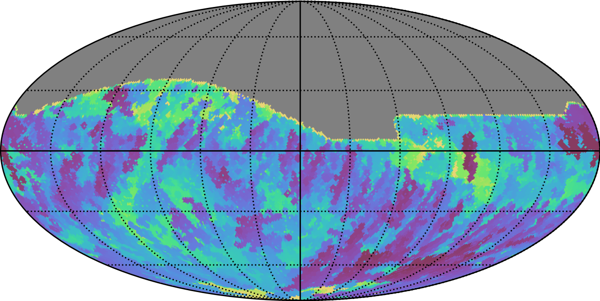
too_elab_r128_d3_gz_v3.4_10yrs All sky r band: Min skyBrightness
