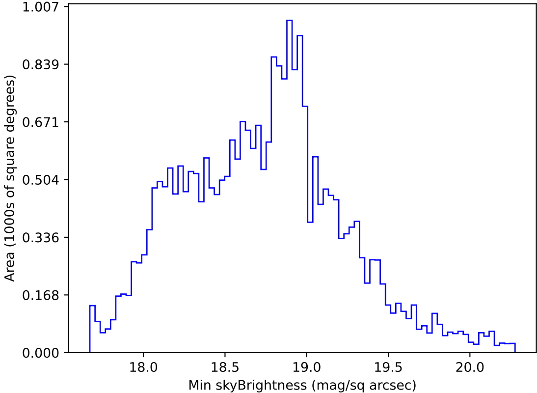
too_elab_r128_d3_gz_v3.4_10yrs All sky r band: Min skyBrightness
