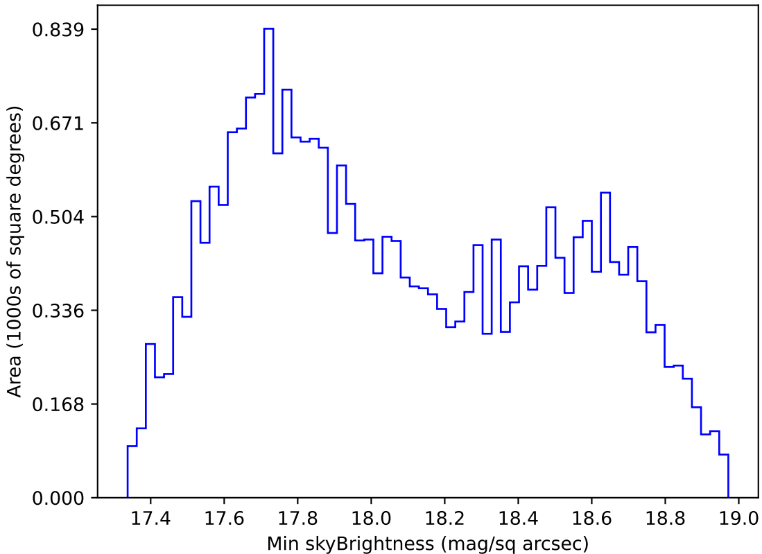
too_elab_r128_d3_gz_v3.4_10yrs All sky i band: Min skyBrightness
