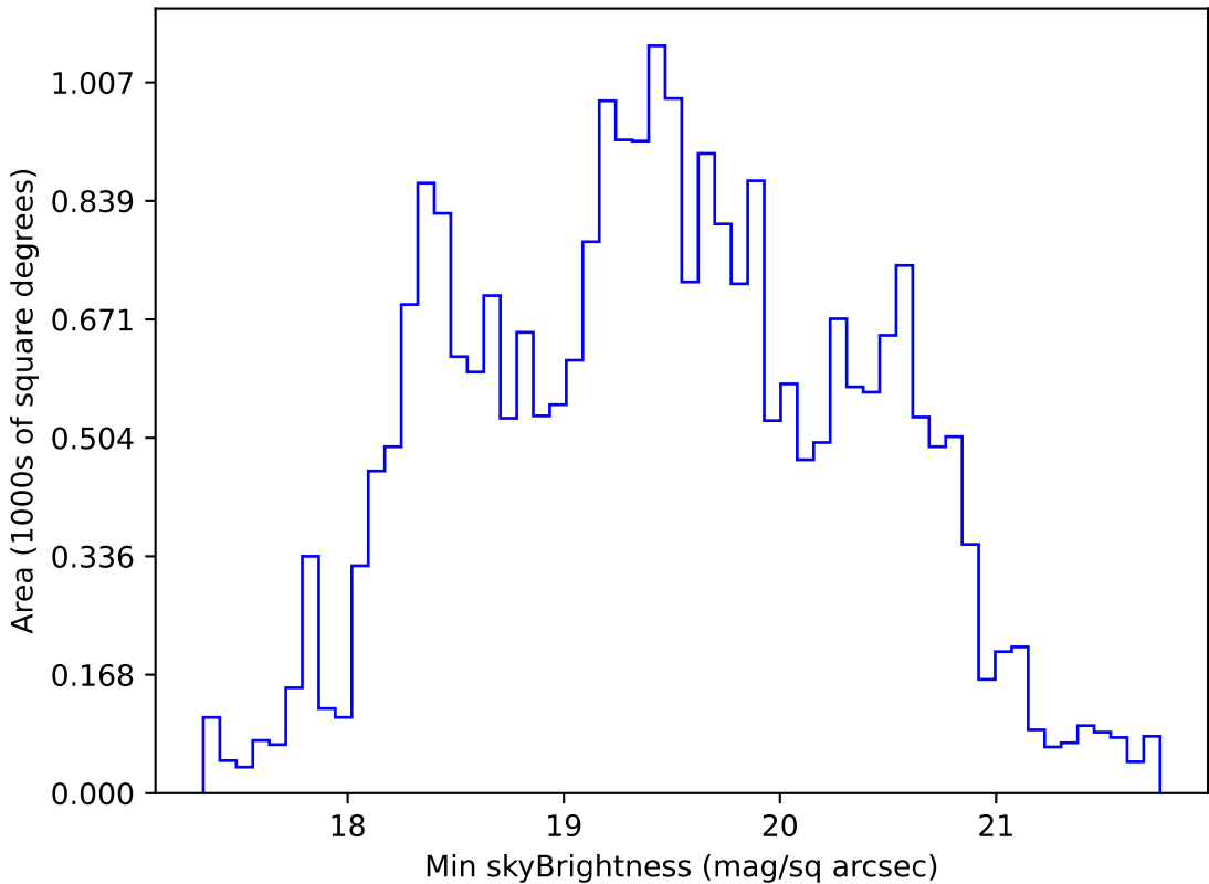
too_elab_r128_d3_gz_v3.4_10yrs All sky g band: Min skyBrightness
