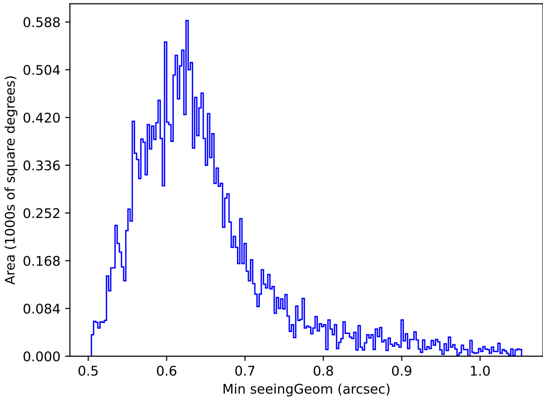
too_elab_r128_d3_gz_v3.4_10yrs Yr 1 z band: Min seeingGeom
