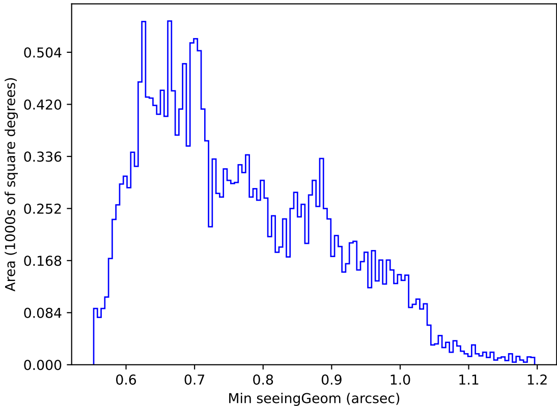
too_elab_r128_d3_gz_v3.4_10yrs Yr 1 u band: Min seeingGeom
