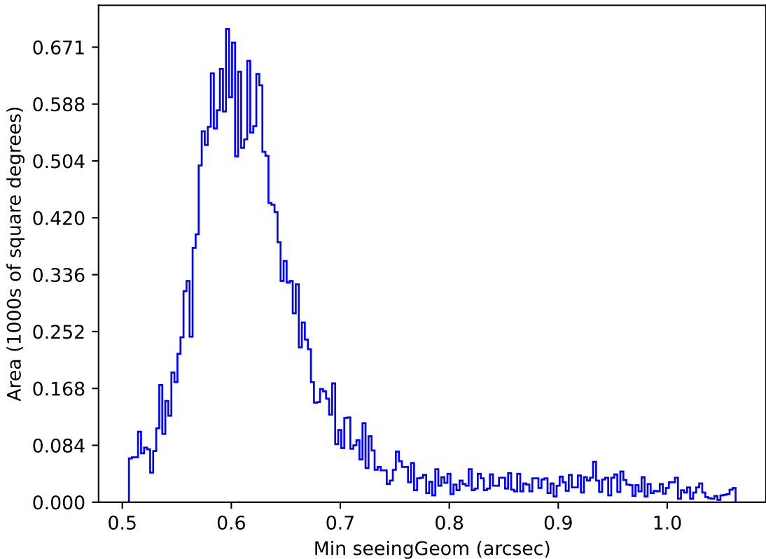
too_elab_r128_d3_gz_v3.4_10yrs Yr 1 r band: Min seeingGeom
