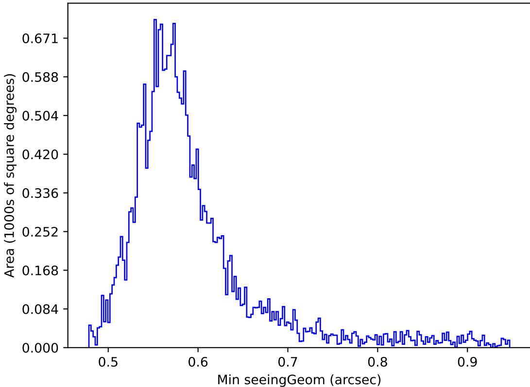
too_elab_r128_d3_gz_v3.4_10yrs Yr 1 all bands: Min seeingGeom
