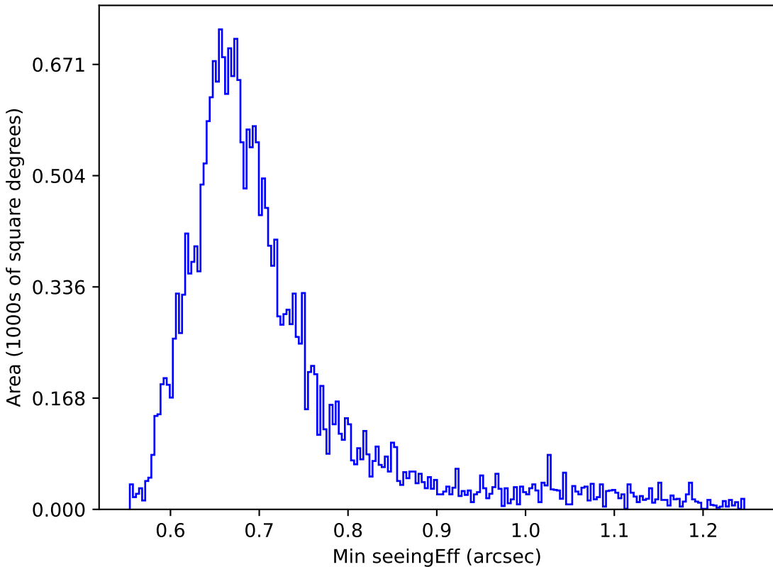
too_elab_r128_d3_gz_v3.4_10yrs Yr 1 i band: Min seeingEff
