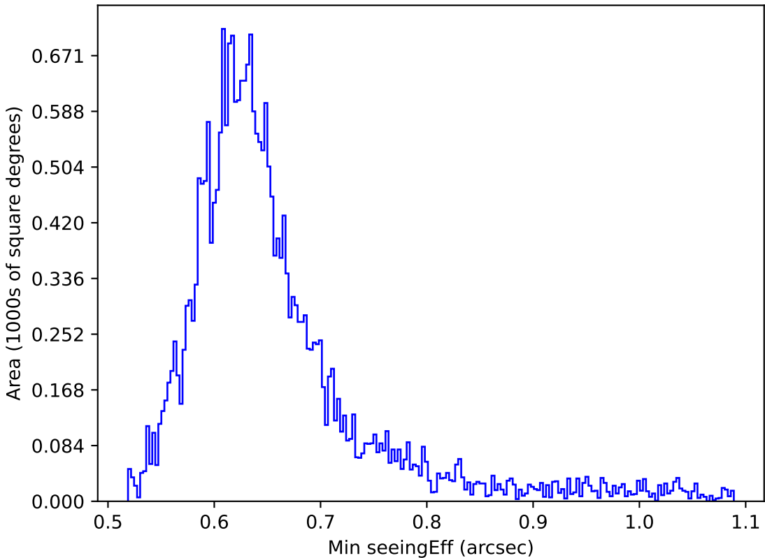
too_elab_r128_d3_gz_v3.4_10yrs Yr 1 all bands: Min seeingEff
