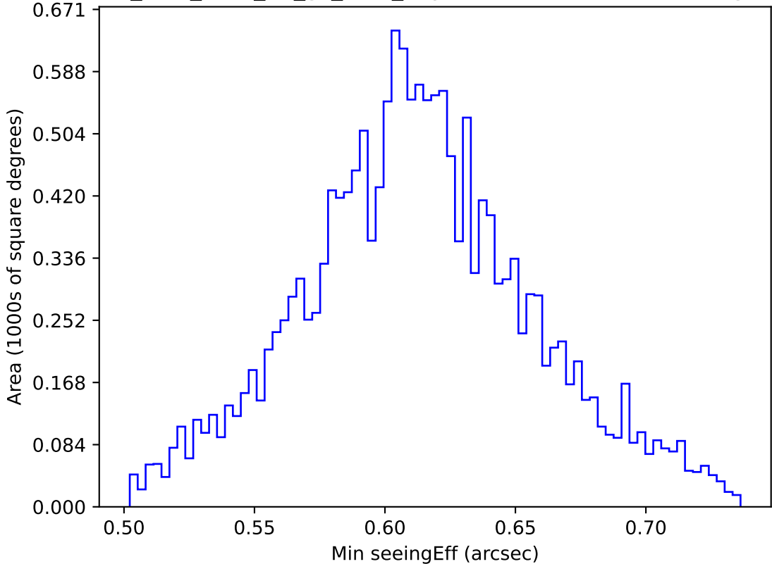
too_elab_r128_d3_gz_v3.4_10yrs WFD z band: Min seeingEff
