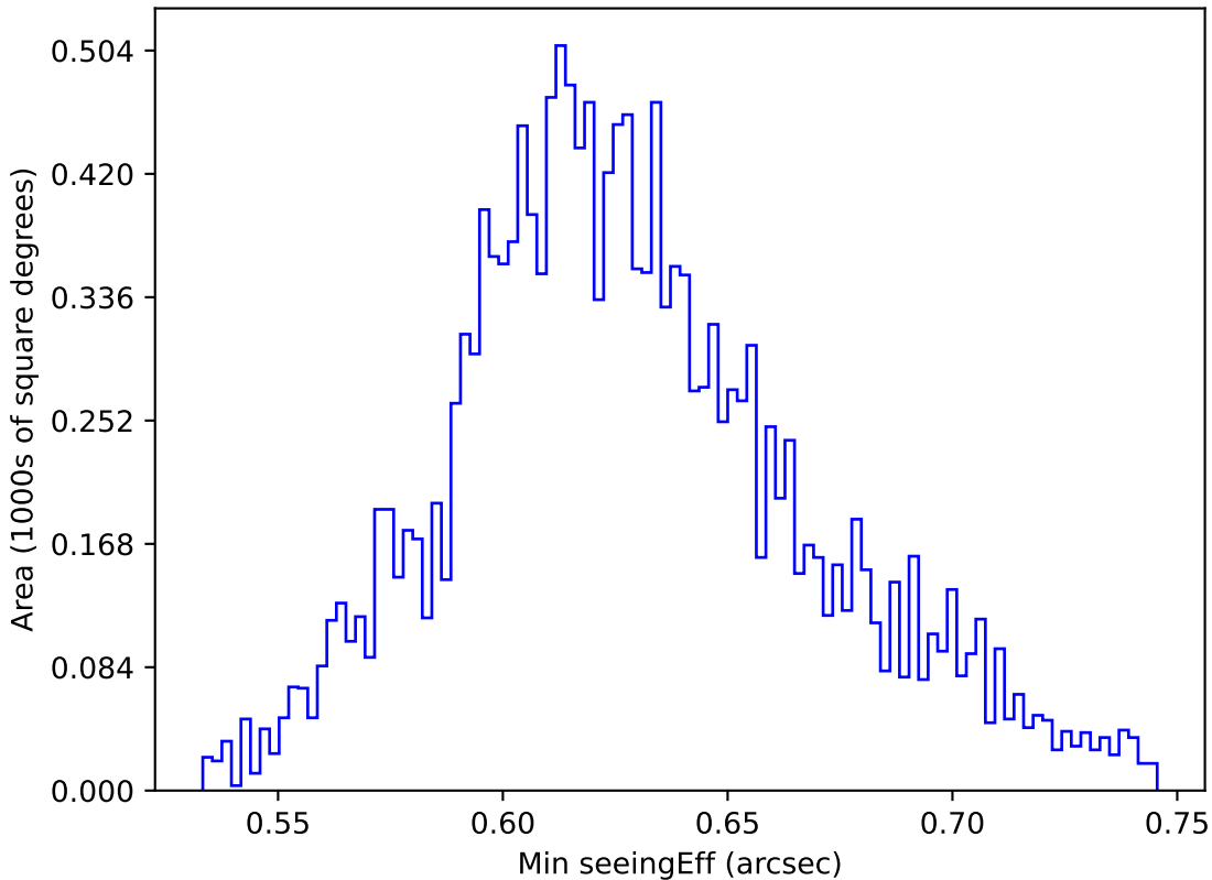
too_elab_r128_d3_gz_v3.4_10yrs WFD y band: Min seeingEff
