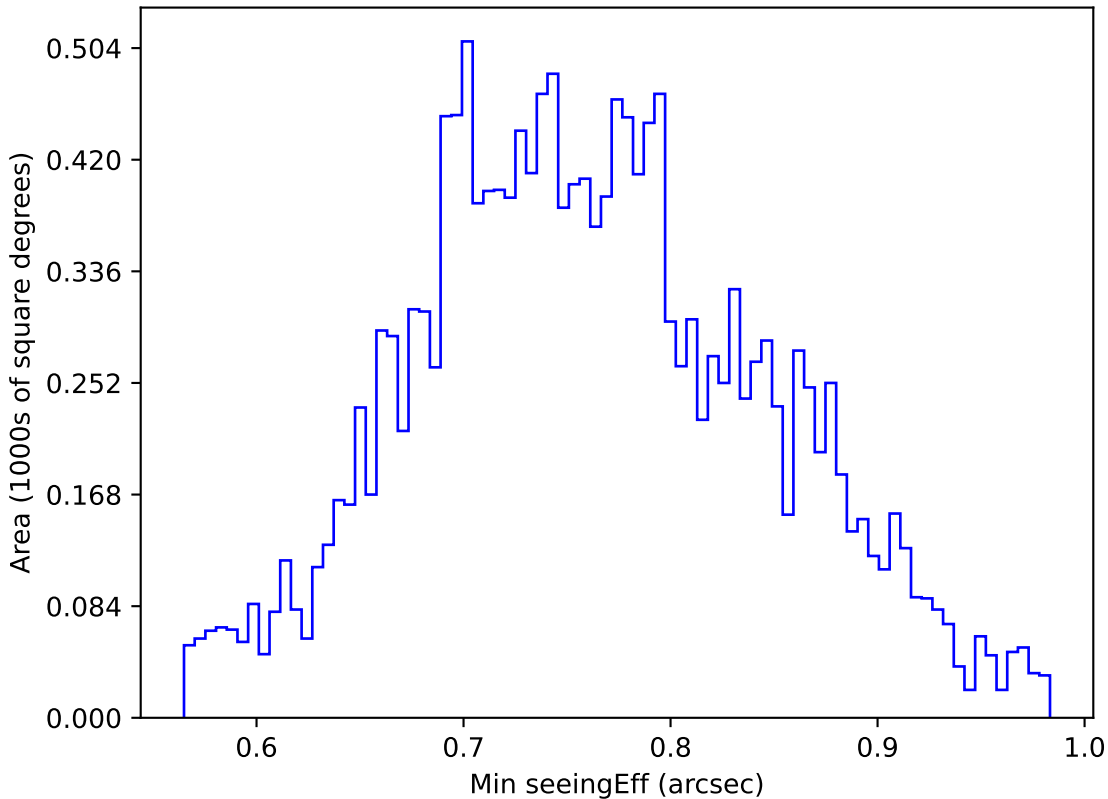
too_elab_r128_d3_gz_v3.4_10yrs WFD u band: Min seeingEff
