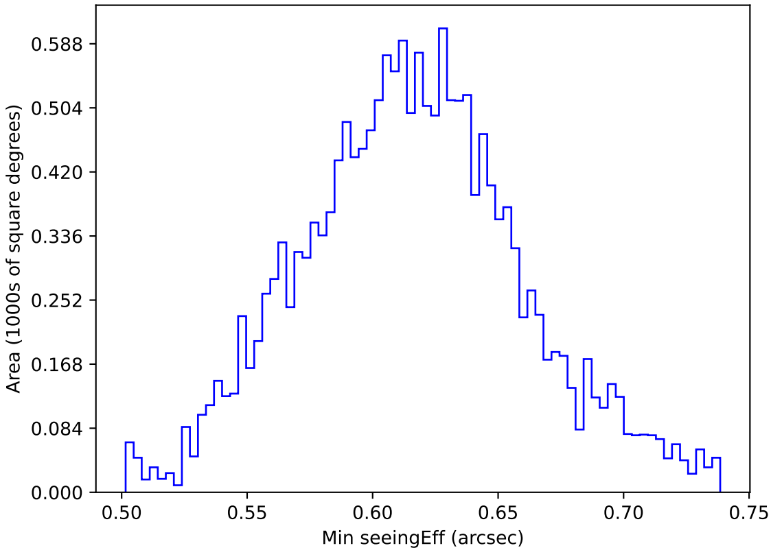
too_elab_r128_d3_gz_v3.4_10yrs WFD r band: Min seeingEff
