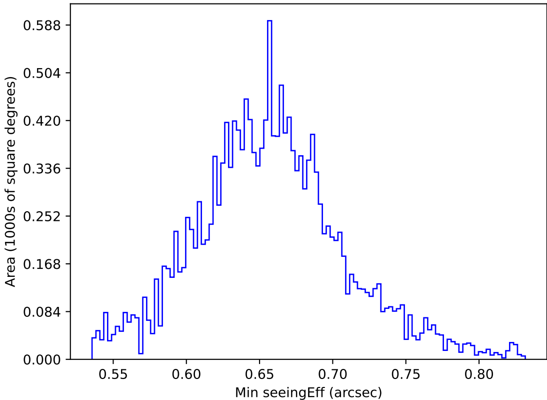
too_elab_r128_d3_gz_v3.4_10yrs WFD g band: Min seeingEff
