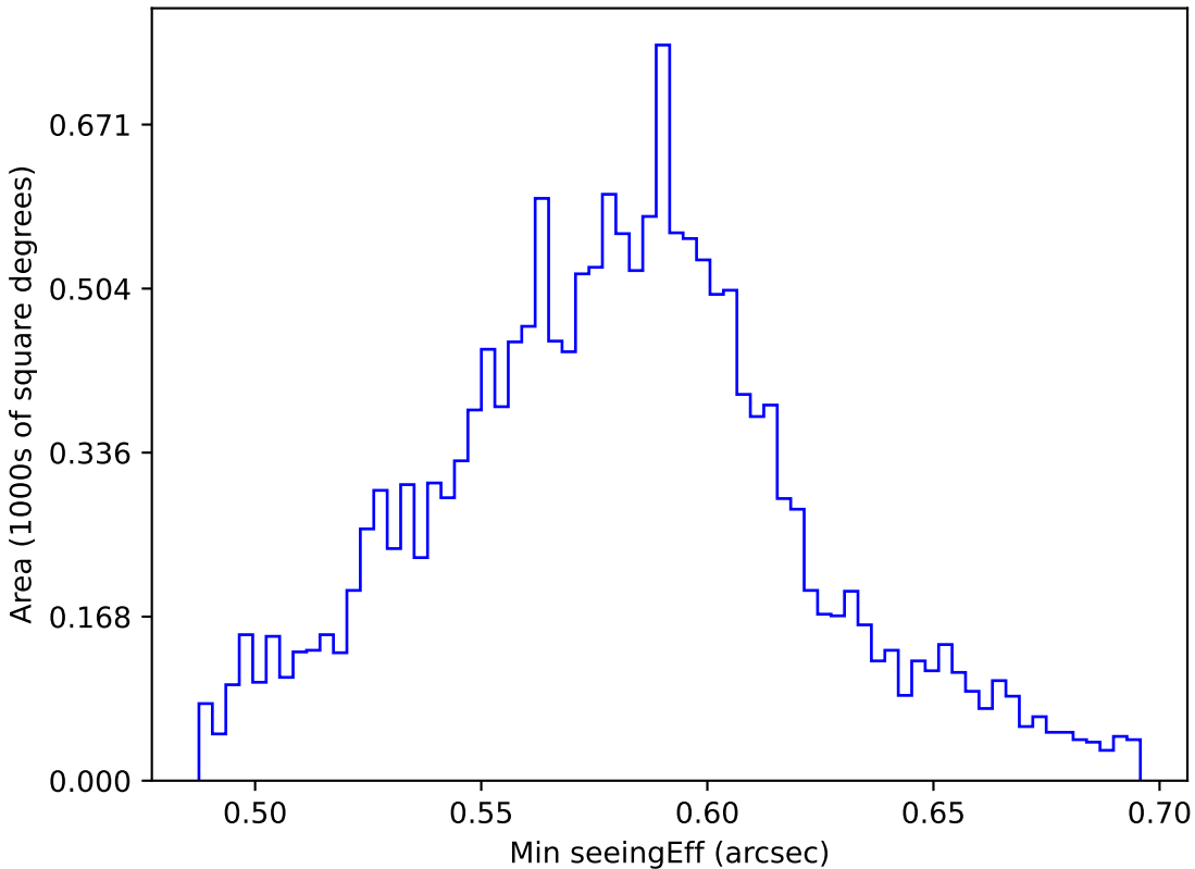
too_elab_r128_d3_gz_v3.4_10yrs WFD all bands: Min seeingEff
