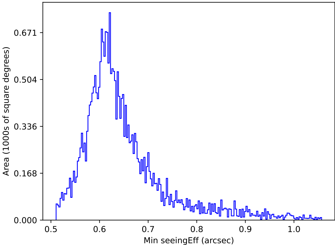
too_elab_r128_d3_gz_v3.4_10yrs All sky z band: Min seeingEff
