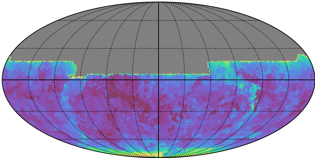
too_elab_r128_d3_gz_v3.4_10yrs All sky y band: Min seeingEff
