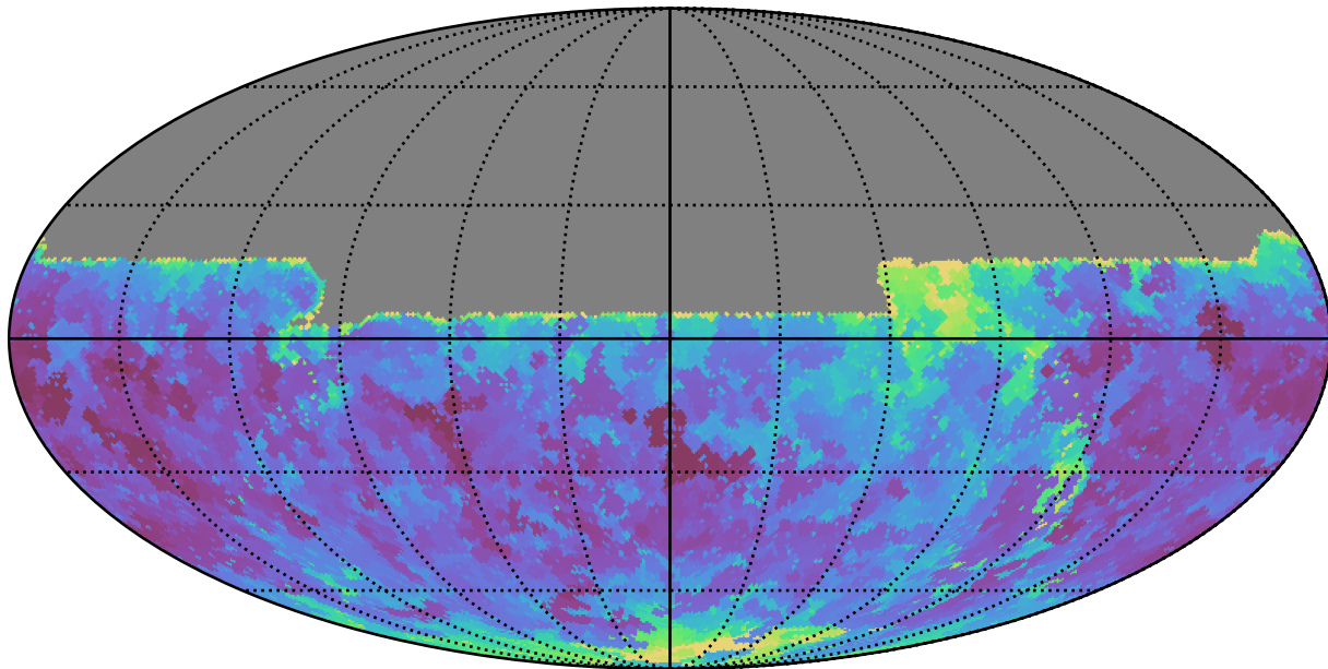
too_elab_r128_d3_gz_v3.4_10yrs All sky u band: Min seeingEff
