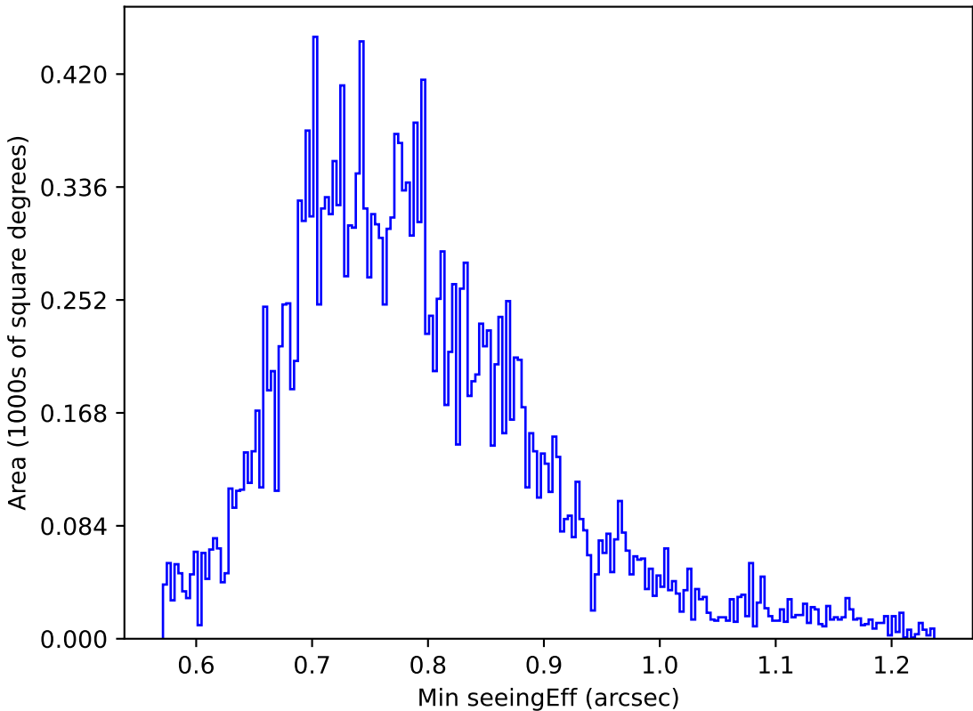
too_elab_r128_d3_gz_v3.4_10yrs All sky u band: Min seeingEff
