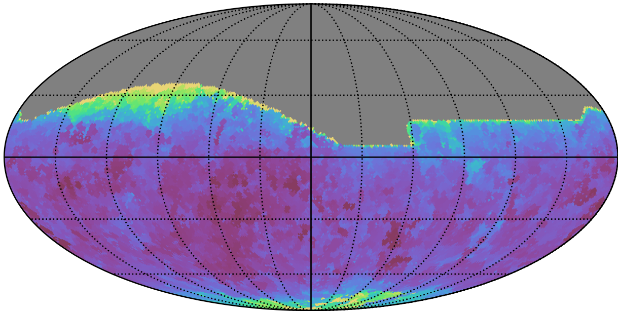
too_elab_r128_d3_gz_v3.4_10yrs All sky r band: Min seeingEff
