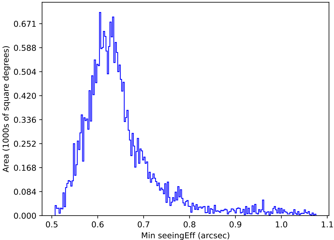
too_elab_r128_d3_gz_v3.4_10yrs All sky r band: Min seeingEff
