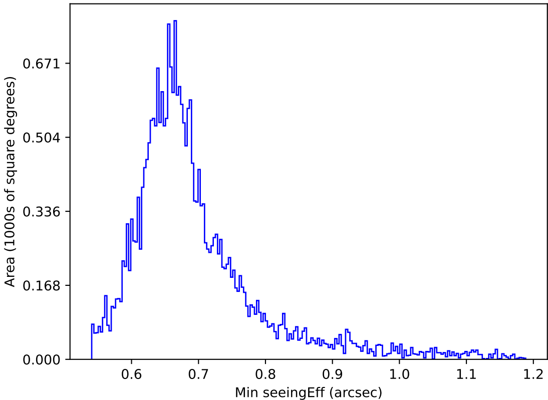
too_elab_r128_d3_gz_v3.4_10yrs All sky g band: Min seeingEff
