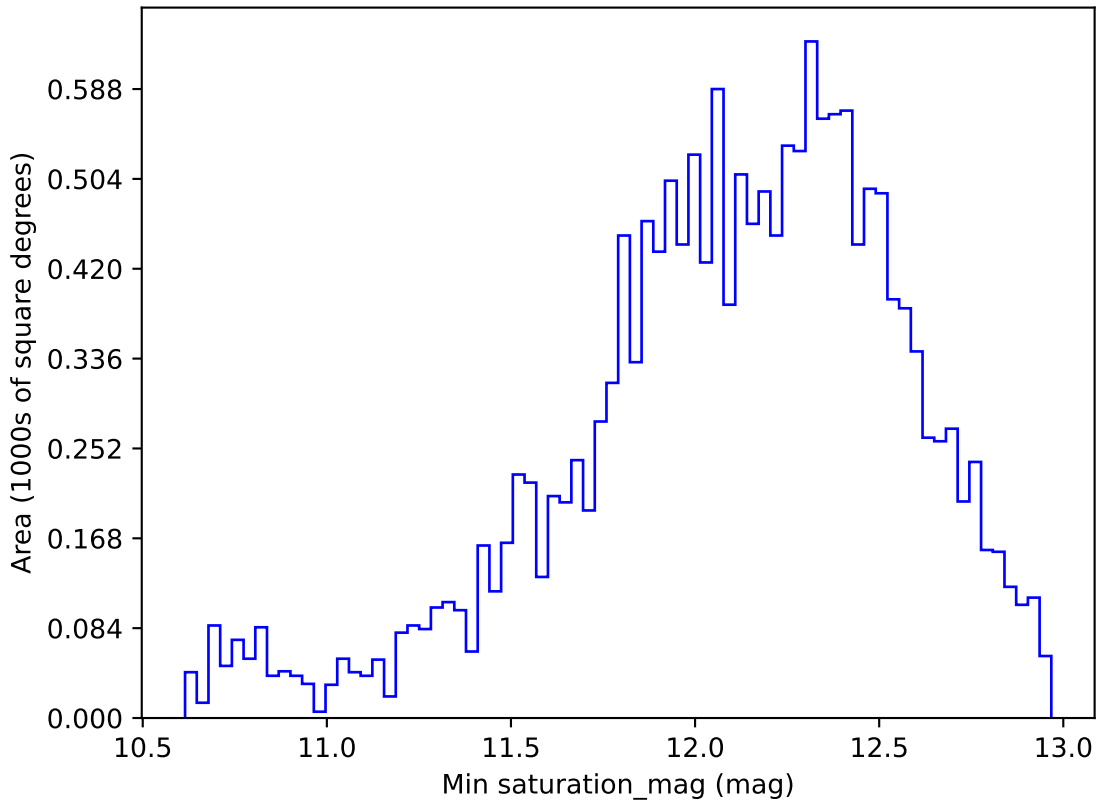
too_elab_r128_d3_gz_v3.4_10yrs WFD z band: Min saturation_mag
