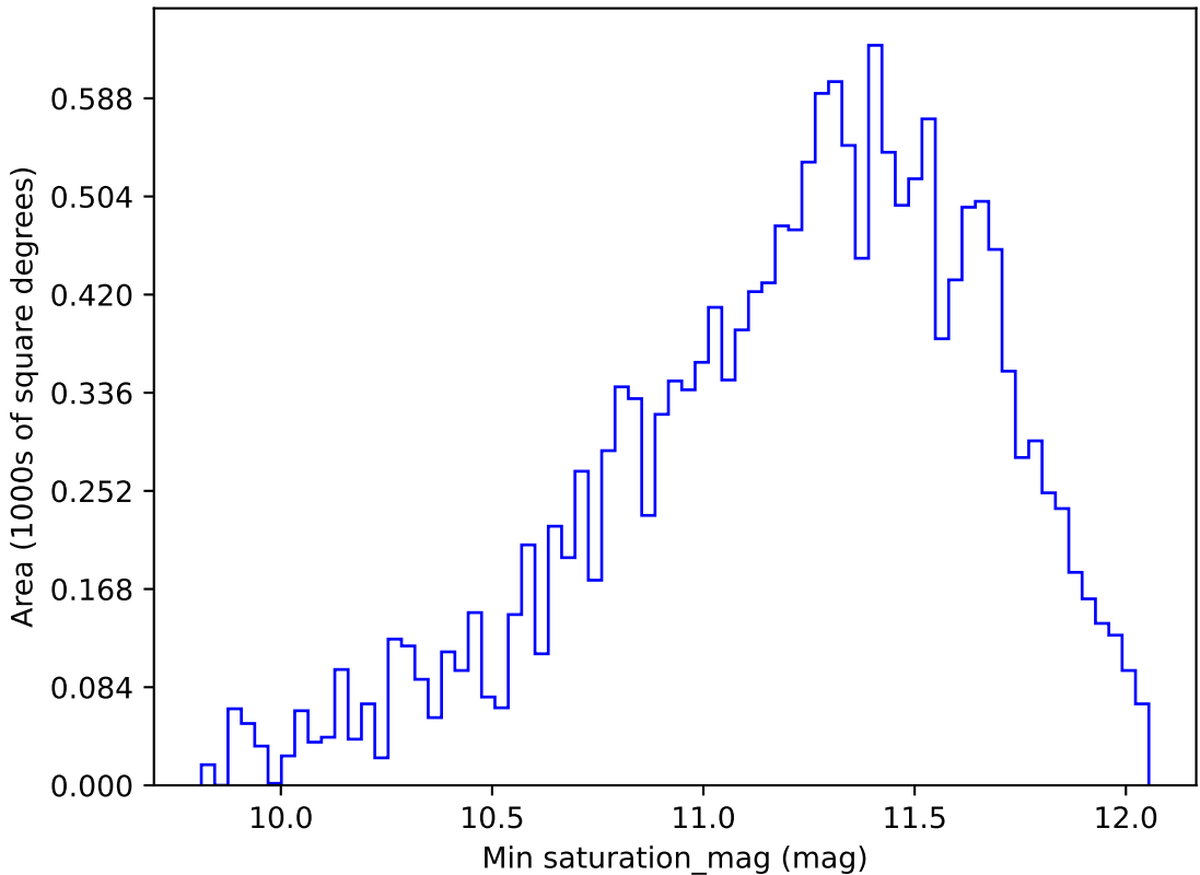
too_elab_r128_d3_gz_v3.4_10yrs WFD y band: Min saturation_mag
