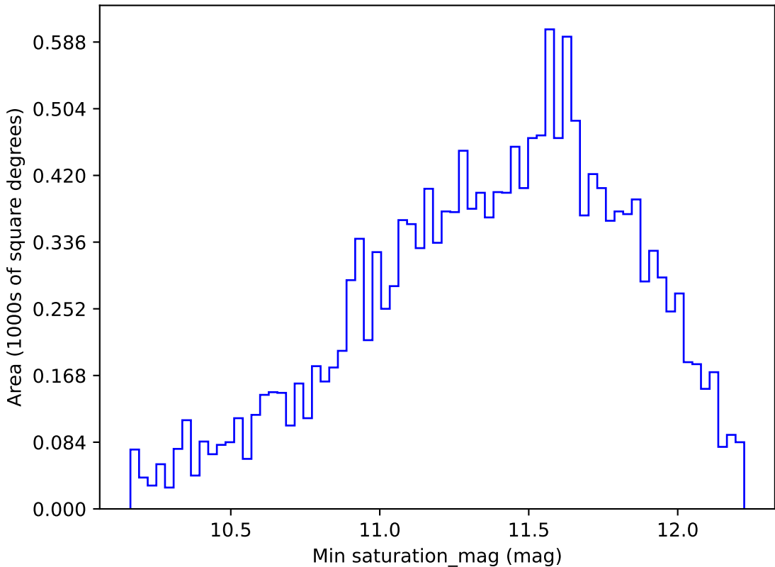
too_elab_r128_d3_gz_v3.4_10yrs WFD u band: Min saturation_mag
