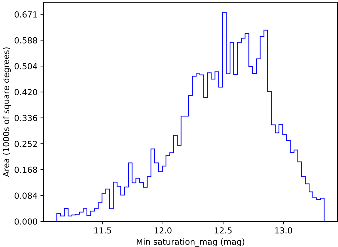
too_elab_r128_d3_gz_v3.4_10yrs WFD r band: Min saturation_mag
