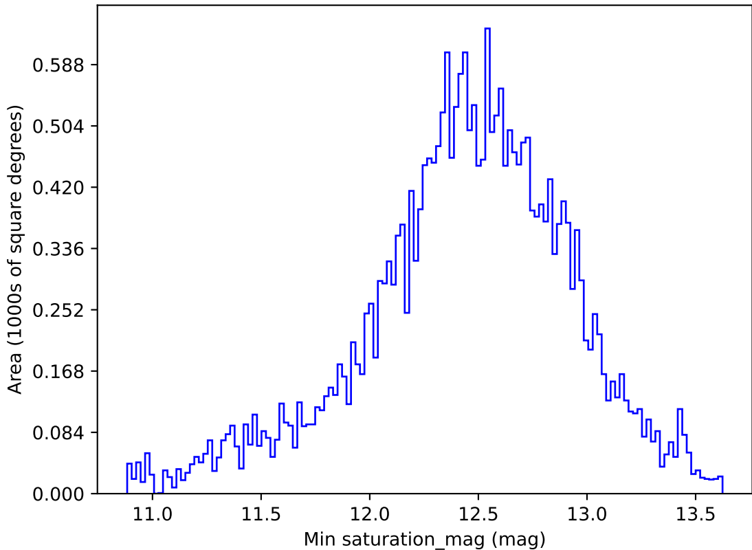
too_elab_r128_d3_gz_v3.4_10yrs All sky i band: Min saturation_mag
