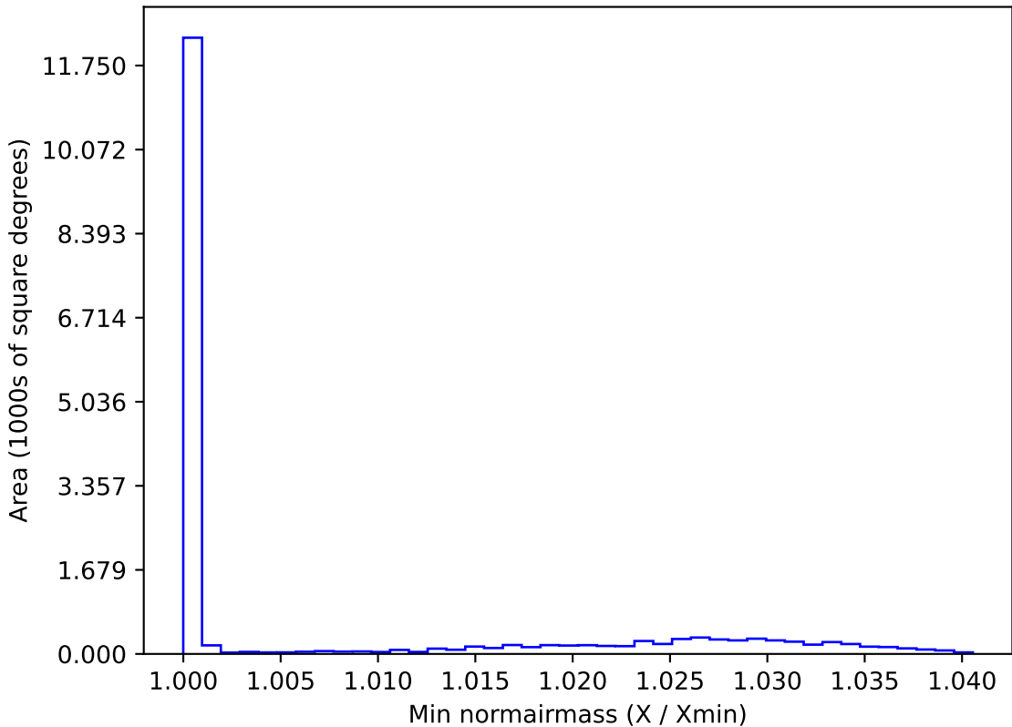
too_elab_r128_d3_gz_v3.4_10yrs WFD y band: Min normairmass
