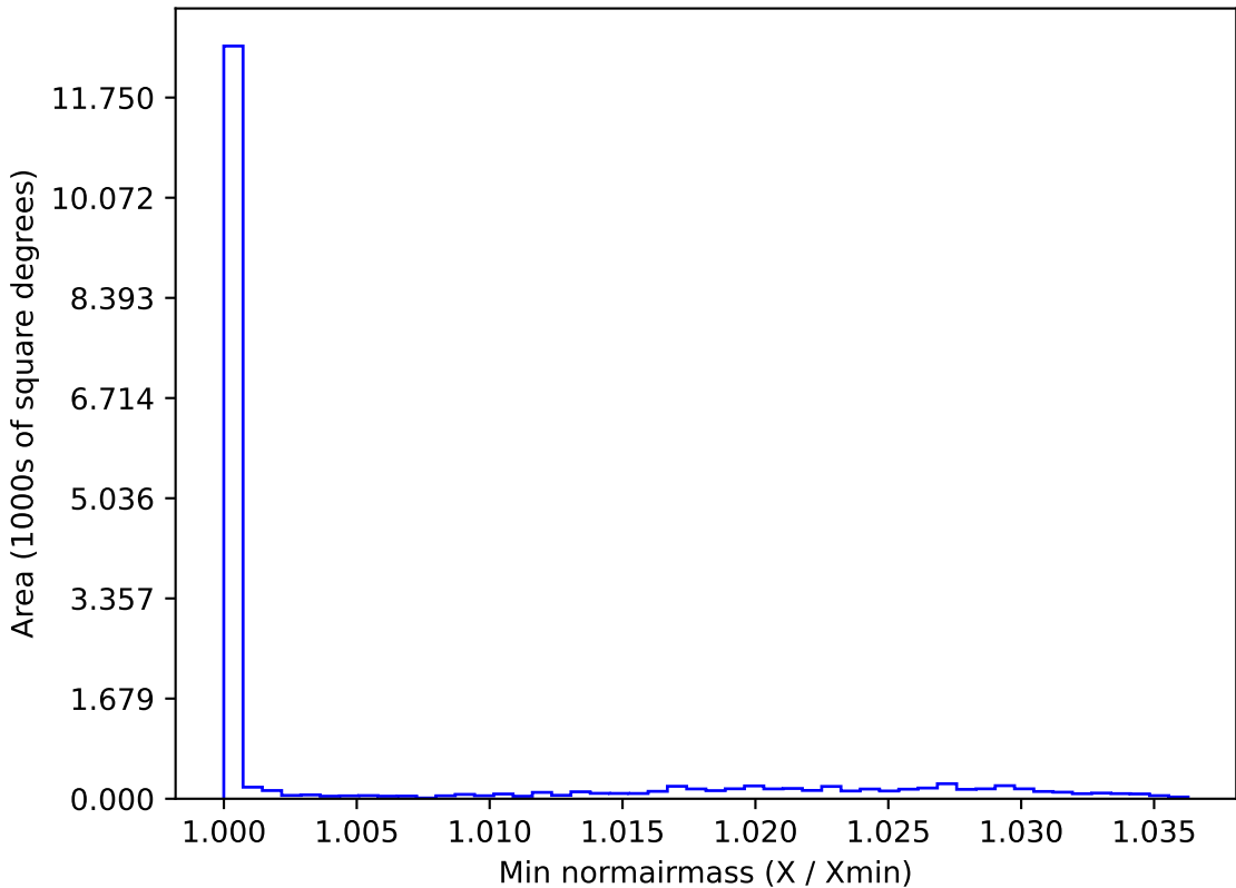
too_elab_r128_d3_gz_v3.4_10yrs WFD r band: Min normairmass
