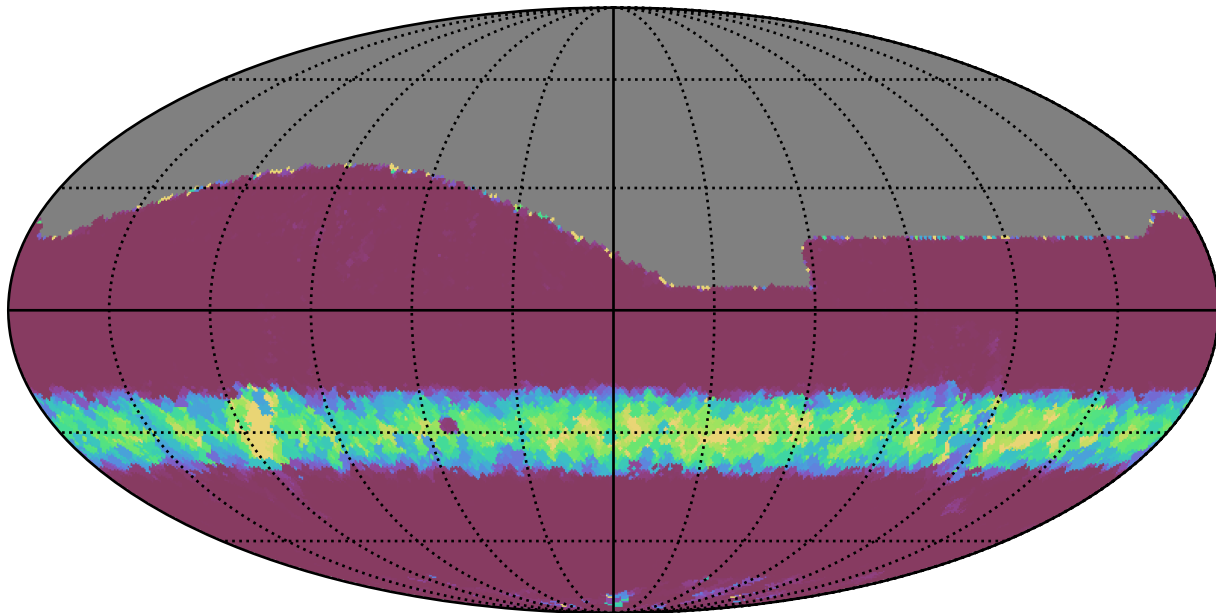
too_elab_r128_d3_gz_v3.4_10yrs All sky r band: Min normairmass
