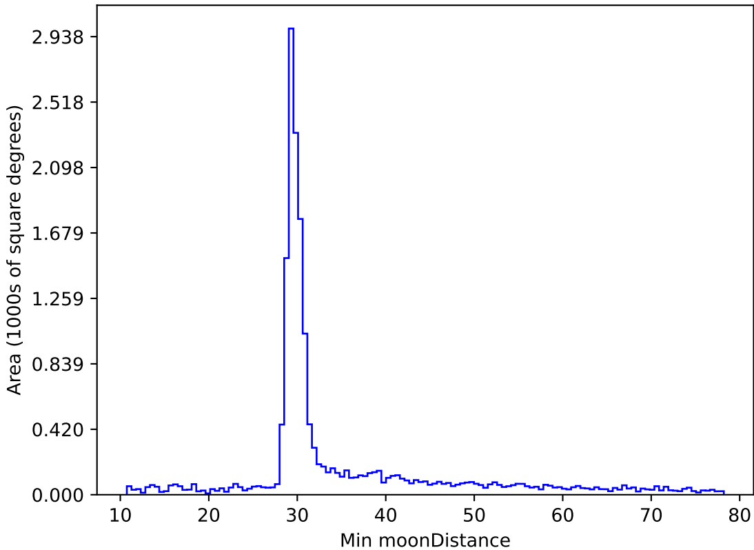
too_elab_r128_d3_gz_v3.4_10yrs WFD z band: Min moonDistance
