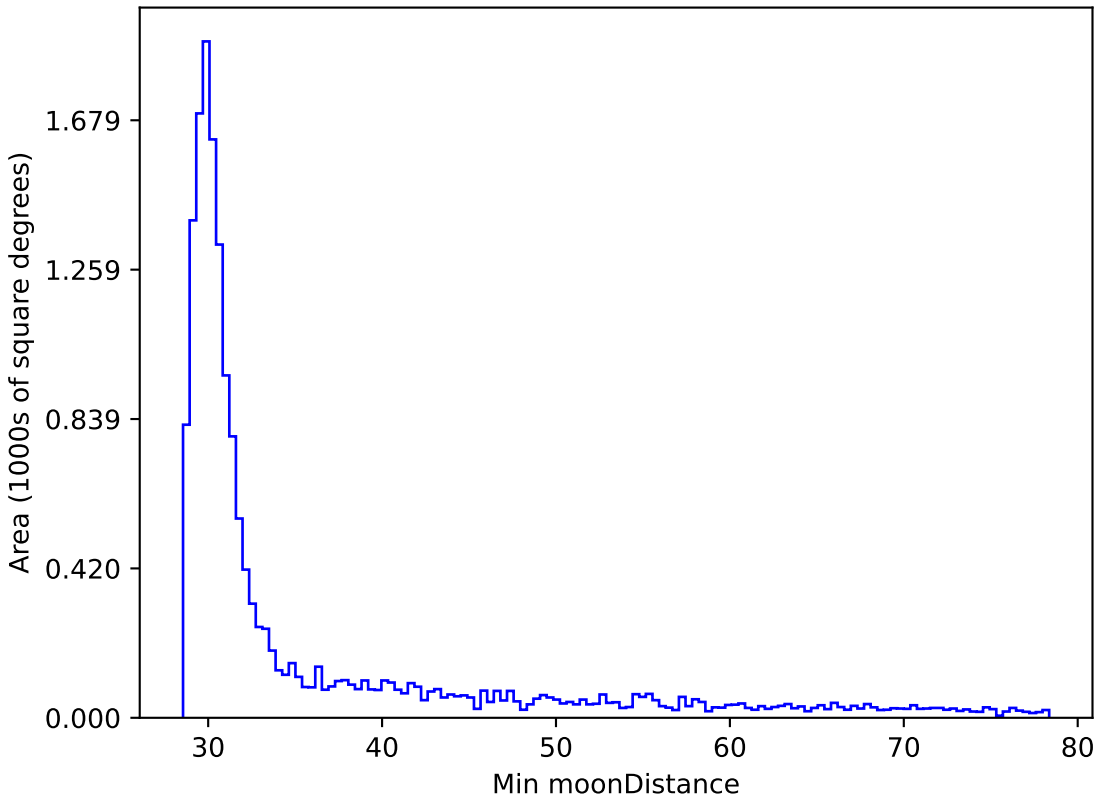
too_elab_r128_d3_gz_v3.4_10yrs WFD i band: Min moonDistance
