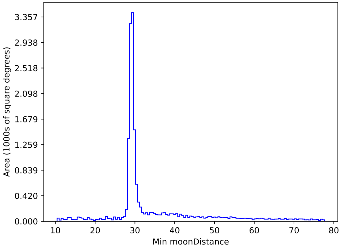
too_elab_r128_d3_gz_v3.4_10yrs WFD all bands: Min moonDistance
