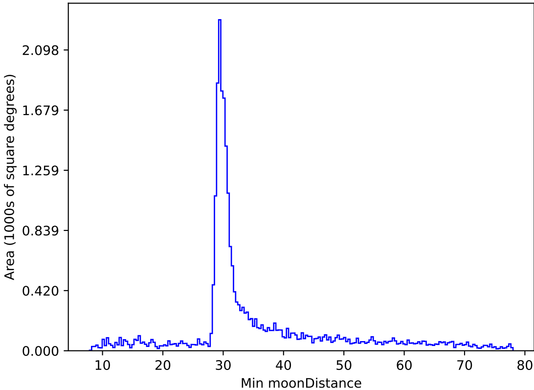
too_elab_r128_d3_gz_v3.4_10yrs All sky z band: Min moonDistance
